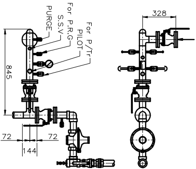
DETAIL: "B" SENSING HEADER
