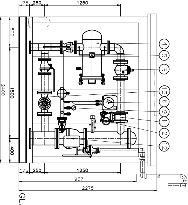
DETAIL: "B" SENSING HEADER
